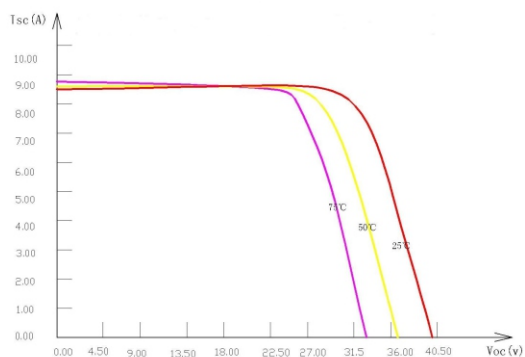
I-V Curves of PV module ZA1ZDNY-260P60 at various cell temperatures
