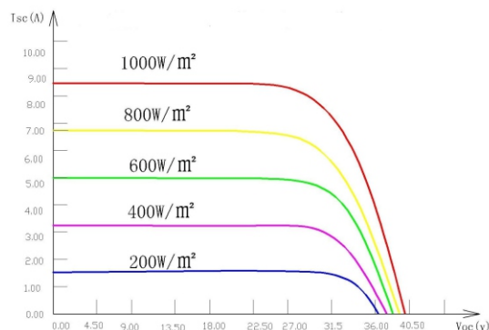
I-V Curves of PV module ZA1ZDNY-260P60 at various solar irradiance
